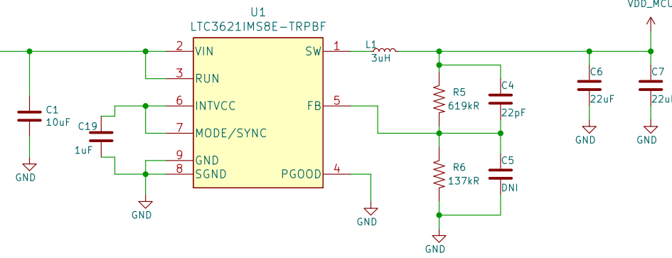
5V to 3V3 Regulator
