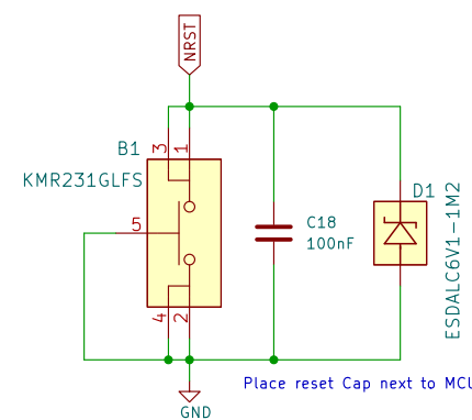
MCU Reset Button
