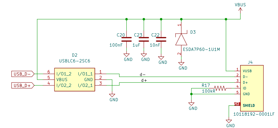
micro USB (Optional)
