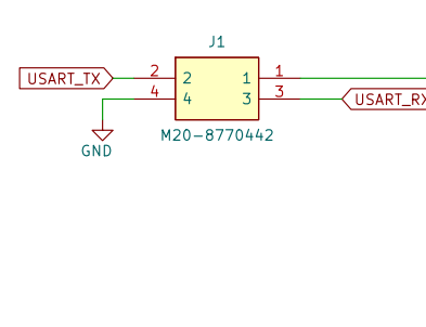
System Connector
