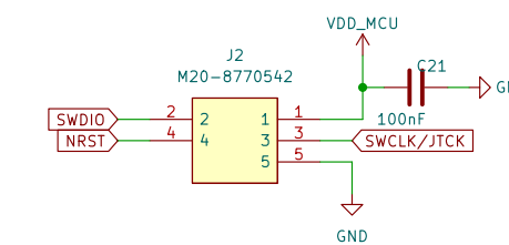
SW Programming
