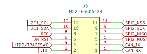
Misc Connections
