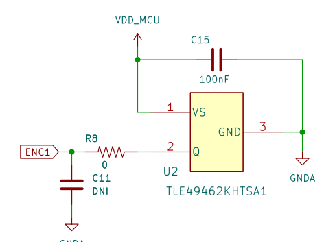
Magnetic Encoder 1
