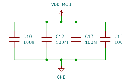
Power Capacitors
