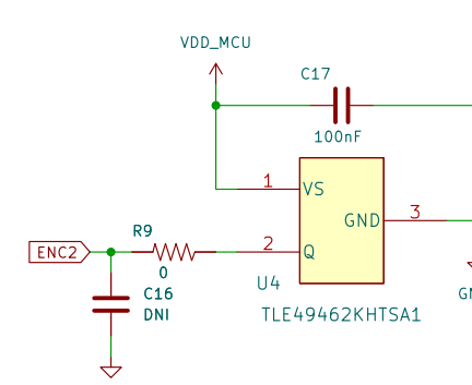
Magnetic Encoder 2
