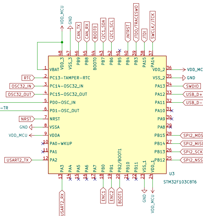
MCU – STM32F103C8T6
