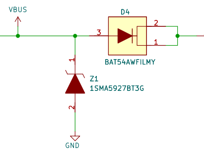
Protection Components
